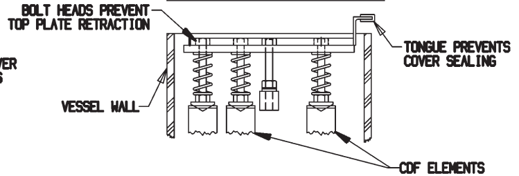
POSITION 1 - BEFORE TIGHTENING
