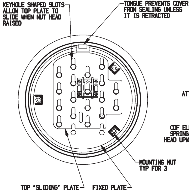
PLAN VIEW - INTERLOCK ASSEMBLY
