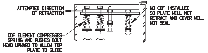
POSITION 3 - FULLY INSTALLED
