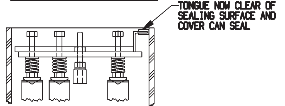
POSITION 3 - FULLY INSTALLED
