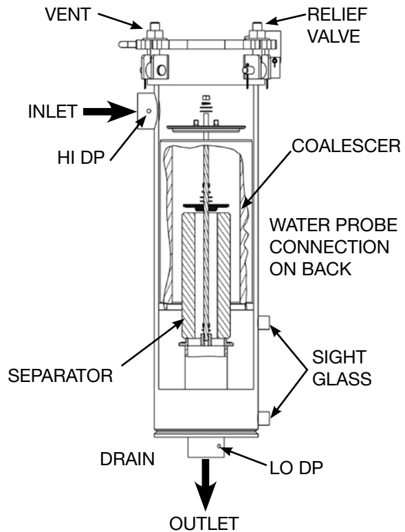
O-81588 and SO-415VX5 Separator
